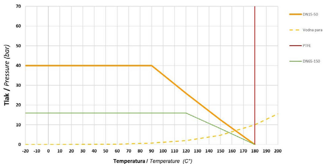
Diagram Tlak/Temperatura / Pressure/Temperature chart Krogelne pipe / Ball valves KPI
