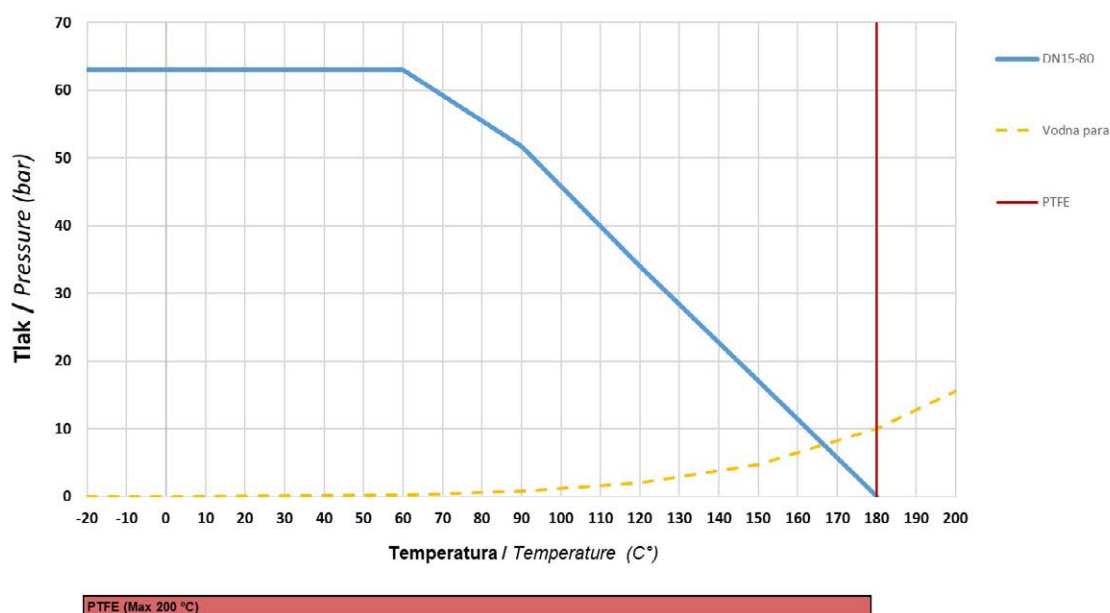
Diagram Tlak/Temperatura / Pressure/Temperature chart Krogelne pipe / Ball valves KPI
